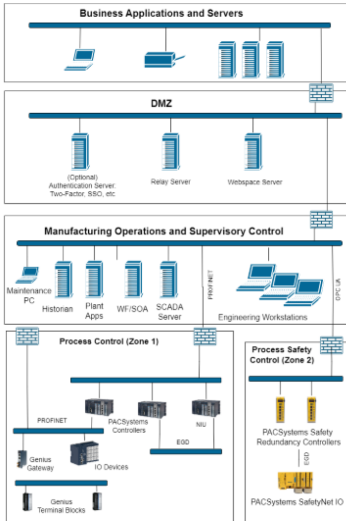
Figure 1: PACSystems Deployed in Purdue Model
